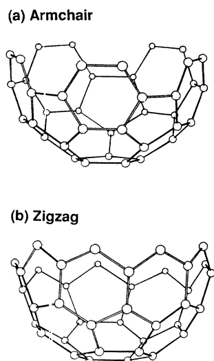
FIG. 1. The caps to graphene tubules formed by cutting the C_{60} molecule along the equatorial plane: (a) the armchair cap normal to a fivefold axis; (b) the zigzag cap normal to a threefold axis.
