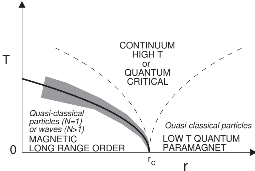
Fig. 8.3. Phase diagram of the theory (8.2) for d < 3 (compare with the large N phase diagram in Fig 5.3. The qualitative features are expected to apply to d > 1 for N = 1 , d \geq 2 for N = 2 , and d > 2 for N \geq 3 . The quantum critical point is at T = 0 with coupling r = r_c (this is also the coupling where s = s_R = 0 ). All properties are however analytic as a function of r at r = r_c for T > 0 . The dashed lines are crossovers at T \sim |r - r_c|^{2\nu} , as is the full line, which is the locus of finite temperature phase transitions at T_c(r) . The shaded region is where the reduced classical scaling functions apply. The region T > T_c(r) , but r < r_c is accessed in our calculation by analytic continuation from r > r_c , T > 0 . The simple perturbative expression in (8.10) can be used in (8.26) for the static susceptibility everywhere in the paramagnetic region, except for the shaded portion. The low T region for r > r_c has a quasi-classical particle description as in Section 4.5.2, and to be discussed in Chapter 9. In the magnetically ordered low T region for r < r_c and N \geq 2 , the long-wavelength spin waves about the ordered state behave classically, while for N = 1 , the amplitude oscillations in \phi_\alpha about its non-zero mean value lead to a quasi-classical particle. As we noted in Fig 7.1, the 'continuum high T ' or 'quantum critical' region is more complex, with thermal and quantum, and particle- and wave-like phenomena playing equal roles. In Section 8.3 we shall show that, to leading order in \epsilon = 3 - d , the low frequency correlators of \phi_\alpha in this region are described an effective quasi-classical wave model; however, the transport of the conserved angular momentum is dominated by higher energy excitations, and requires a particle-like description in a quantum Boltzmann equation which will be discussed in Chapter 9.
