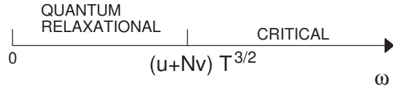
Fig. 16.2. Crossovers as a function of frequency, \omega , in the regions of Fig 16.1 of the metallic spin glass. The low T Fermi liquid region is on the paramagnetic side ( s > 0 ).
