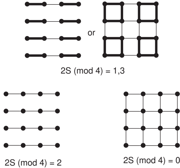
Fig. 13.2. Quantum paramagnetic ground states of the weakly frustrated square lattice antiferromagnet as a function of 2S(\text{mod } 4) . The values of P_{ij} on the nearest neighbor links are schematically indicated by the different kinds of lines on the links; those on thick lines are larger than those on the thin lines, and weakest are on the empty links.
