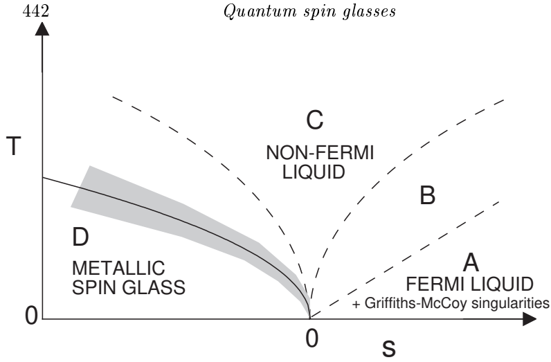
Fig. 16.1. Mean field phase diagram of a metallic spin glass as a function of the ground state tuning parameter s and temperature T . The T = 0 state is a metallic spin glass for s < 0 and a disordered, paramagnetic Fermi liquid for s > 0 . The full line is the only thermodynamic phase transition, and is at s = s_c(T) or T = T_c(s) given in (16.44). The quantum critical point is at s = 0, T = 0 . The dashed lines denote crossovers between different finite T regions of the quantum field theory (16.14): the low T regions are A, B (on the paramagnetic side) and D (on the ordered side), while the high T region (C) displays ‘non-Fermi liquid’ behavior. The crossovers on either side of C, and the spin glass phase boundary T_c(s) , all scale as T \sim |s|^{2/3} ; the boundary between A and B obeys T \sim s . The shaded region has classical critical fluctuations described by theories of the type discussed by Refs [54, 150].
