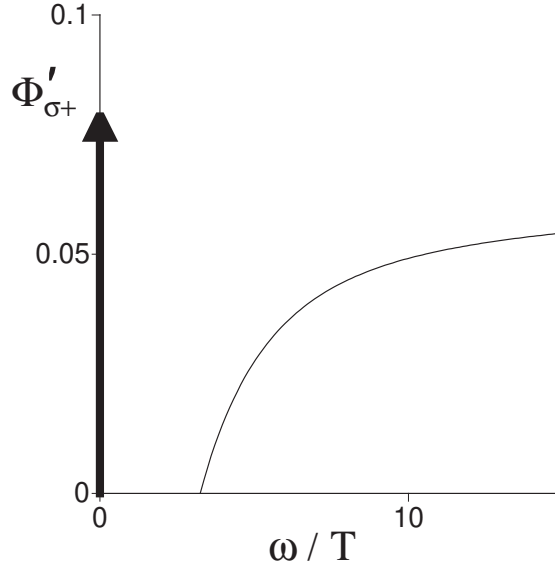
Fig. 9.2. The real part, \Phi'_{\sigma+} , of the universal scaling function \Phi_{\sigma+} in the high T limit ( T \gg \Delta_{\pm} ) (see (9.17)) at the one loop level. The numerical values are obtained from (9.26) and (9.27) with d = 2 ( \epsilon = 1 ). There is a delta function precisely at \omega/T = 0 represented by the heavy arrow: the weight of this delta function is given in (9.28) and (9.29). The delta function contributes to \sigma_I , and the higher frequency continuum to \sigma_{II} .
