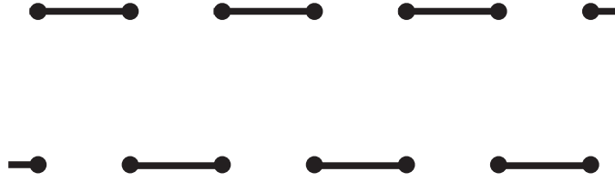
Fig. 14.4. Schematic of the two spin-Peierls ground states of H_{12} . The thick lines represent larger values of \langle \vec{\sigma}_i \cdot \vec{\sigma}_{i+1} \rangle , while the unmarked near-neighbor pairs have smaller values.
