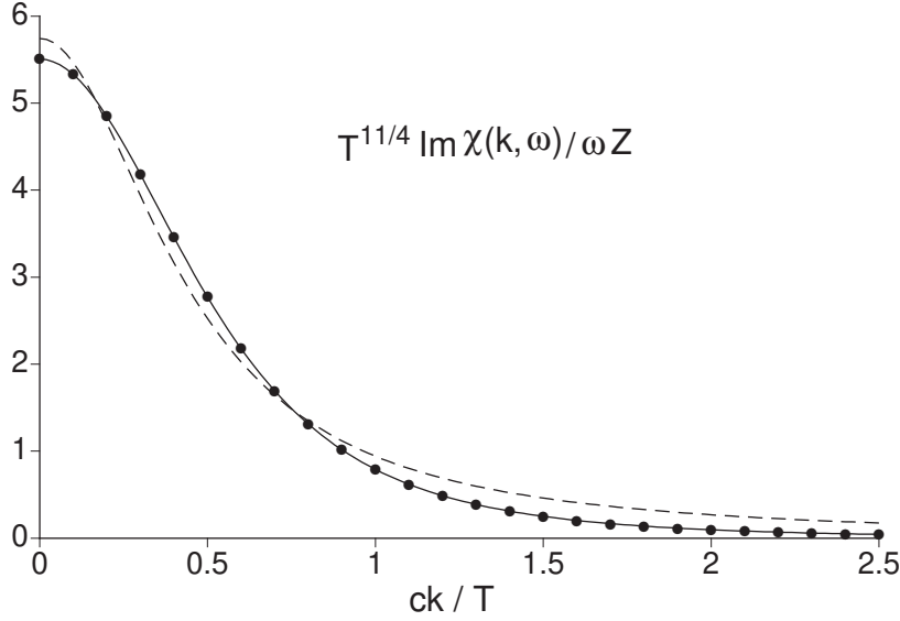
Fig. 4.11. Comparison of the predictions of (4.114) (dots) and (4.115) (solid line) for \text{Im}\chi(k, \omega)/\omega at \omega = 0 as a function of ck/T . The best fit parameters in (4.116) were used. The function (4.115) yields the square of a Lorentzian as a function of k ; a best fit by just a Lorentzian is also shown (dashed line), and is much poorer.
